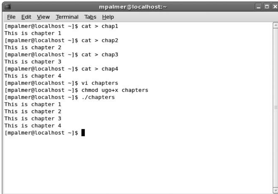
Figure 6-12 Executing the chapters shell script
