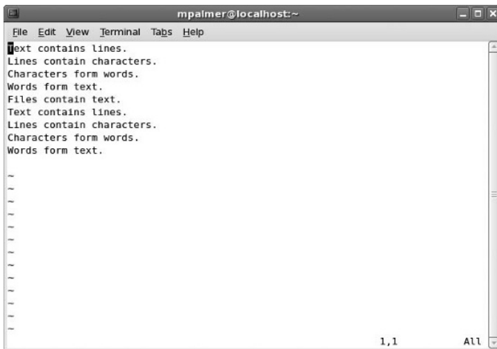
Figure 3-8 File after deleting the first line
