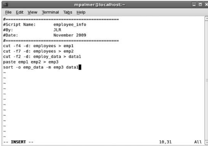
Figure 4-6 Sample script file
