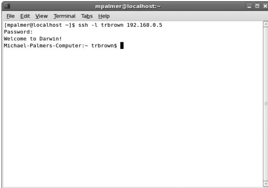
Figure 1-13 Using SSH from a GNOME terminal window to access another account on a remote UNIX/Linux computer
