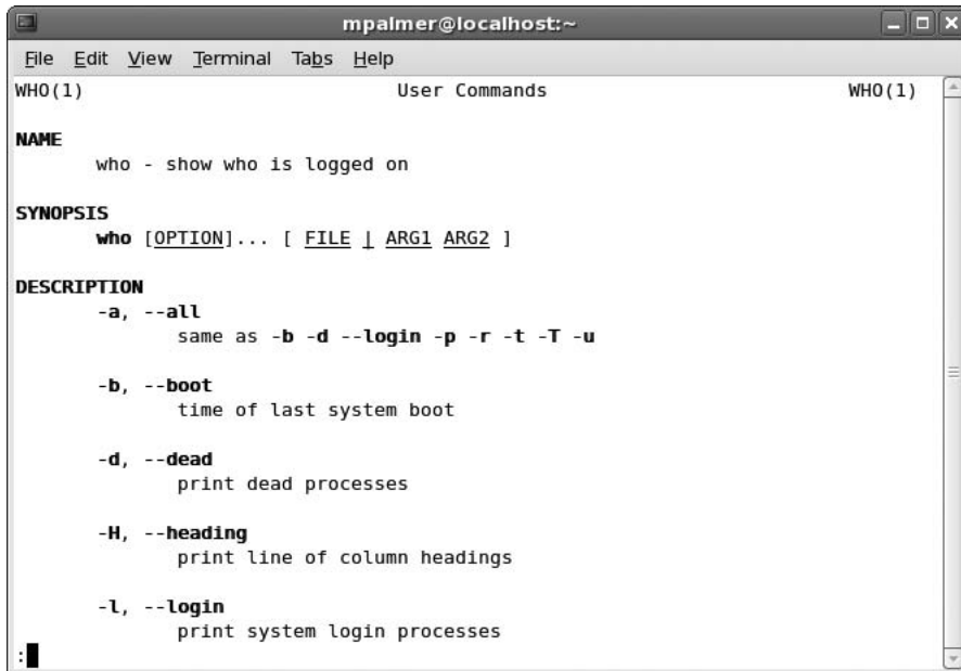
Figure 1-16 Using man to find out more about the who command
