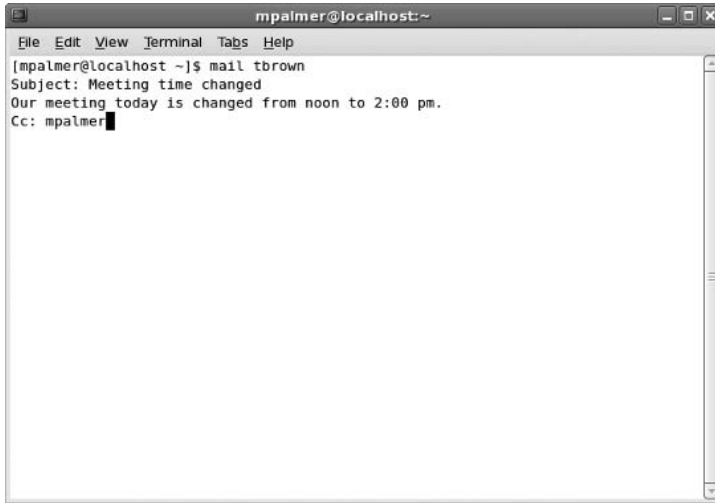
Figure 8-6 Using the mail command
