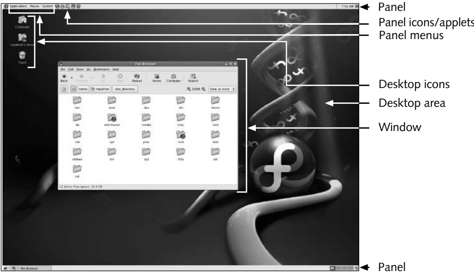
Figure 11-4 Major GNOME components in Fedora
