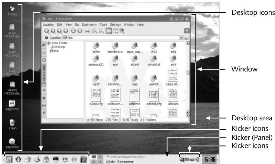
Figure 11-9 Major KDE components
