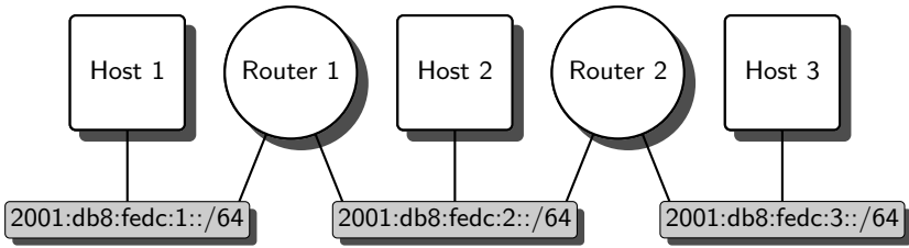
Fig. 7.1. Autoconfiguration and ICMPv6 redirects
