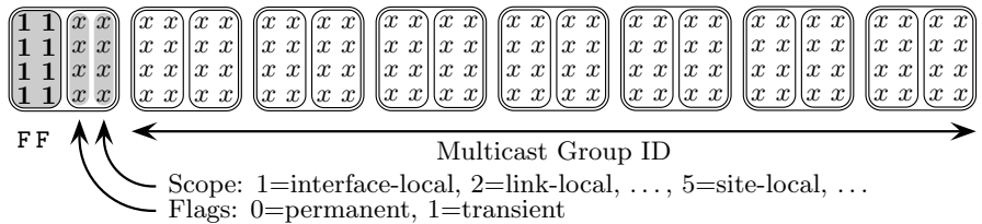
Fig. 3.4. Multicast addresses
