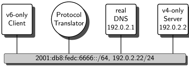
Fig. 10.1. A protocol translation test setup
