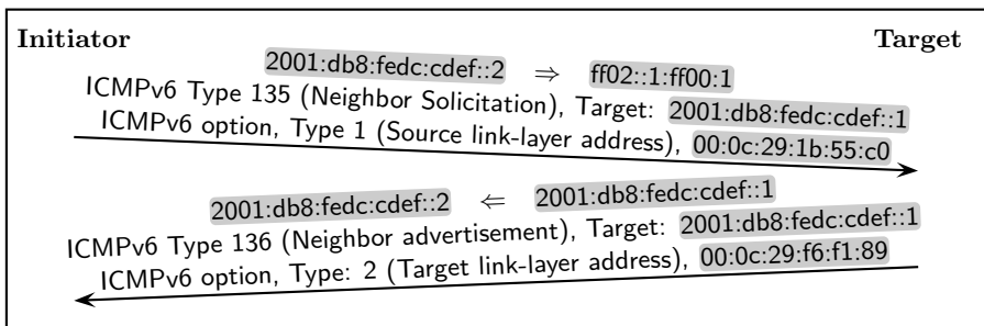
Fig. 4.2. Neighbor discovery as an ARP successor
