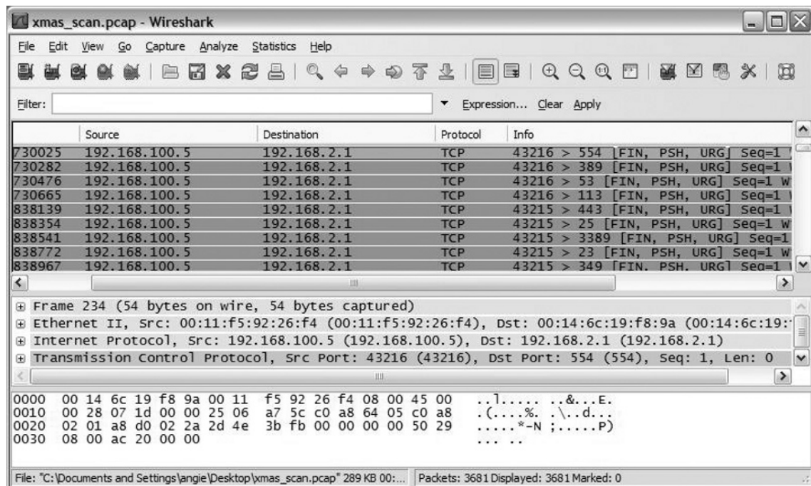
Figure 8.6 XMAS Scan
