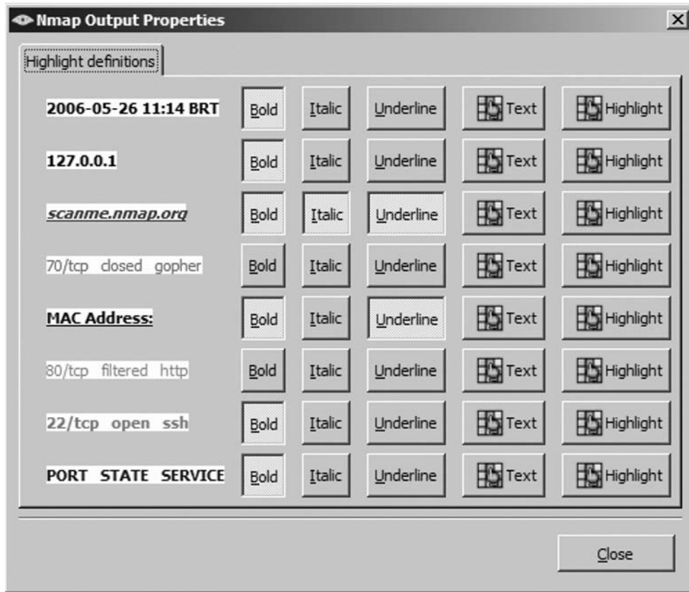
Figure 5.5 Highlight Definitions
