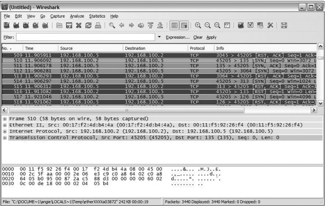
Figure 8.5 SYN Scan
