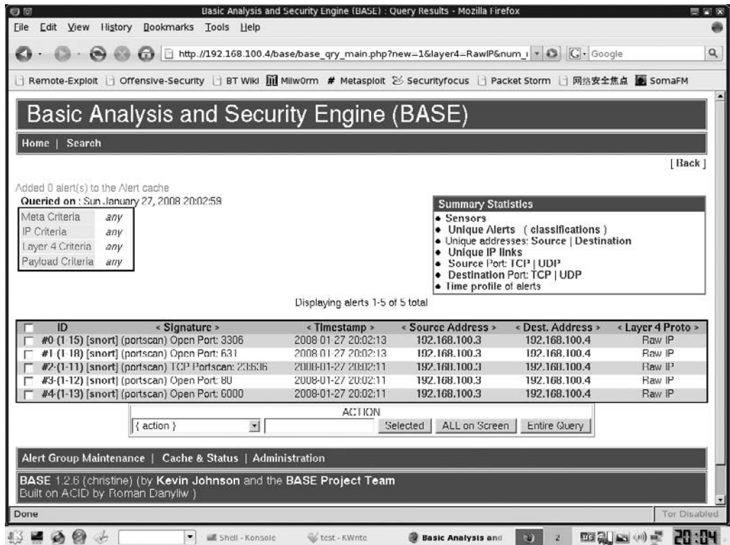
Figure 8.4 BASE Alerts
