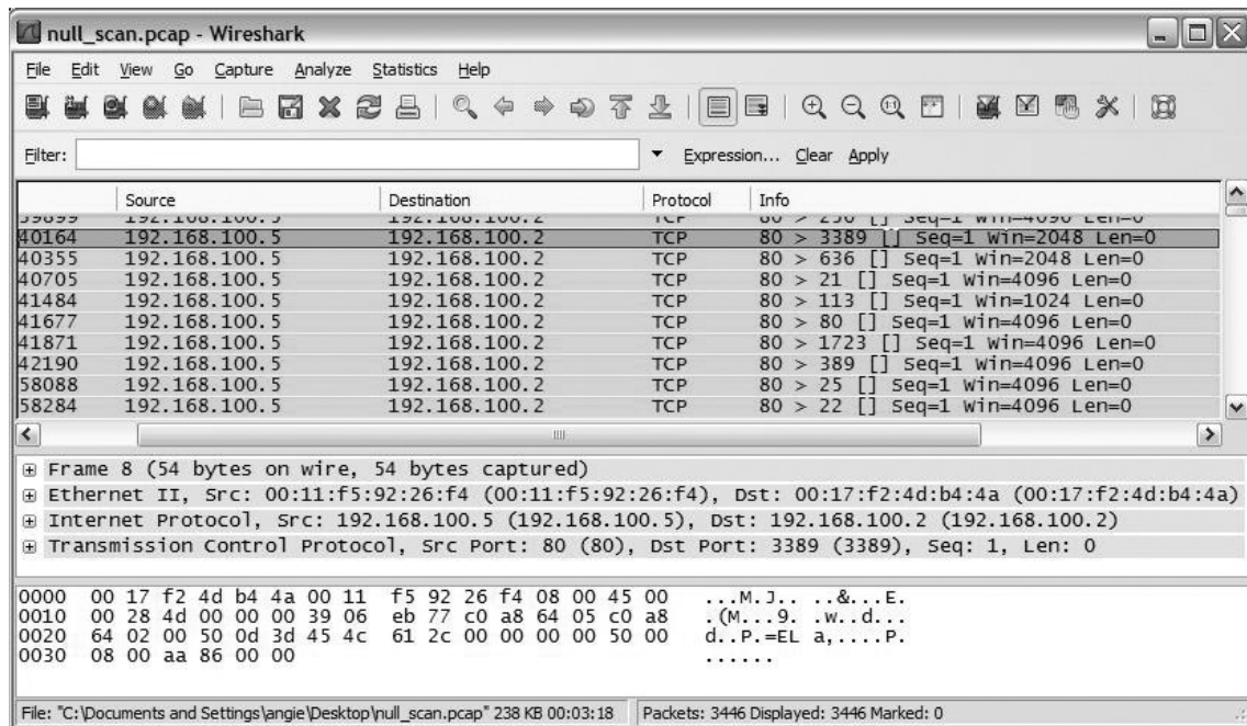
Figure 8.7 Null Scan
