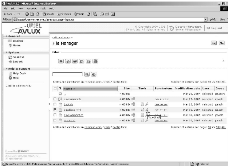
Fig. 12.35 Selecting database.yml
